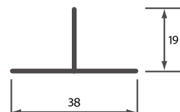
Low profile Bottom 'T' Track Low security option SeceuroGuard 1000 only
